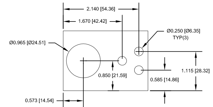
PLITKA 12HP ARCADE v2.1 (ARCADE BUTTON, 2 JACKS, 1 POT) BTN MASHR
