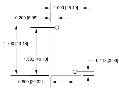
PLITKA 1U 5HP
